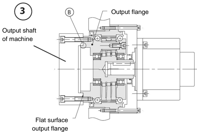
Fig. 17 F4CF-D installation example 2
