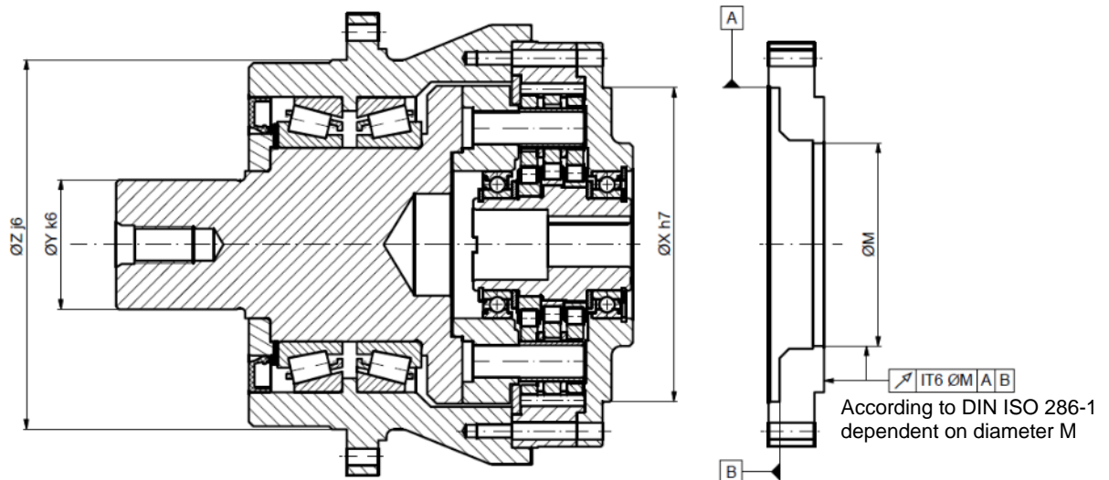
Fig. 13 F3C-A assembly tolerances
