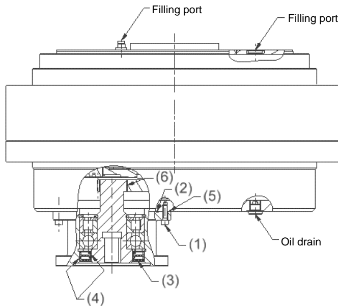
Fig. 4 Oil change vertical mounting position (output upwards)
