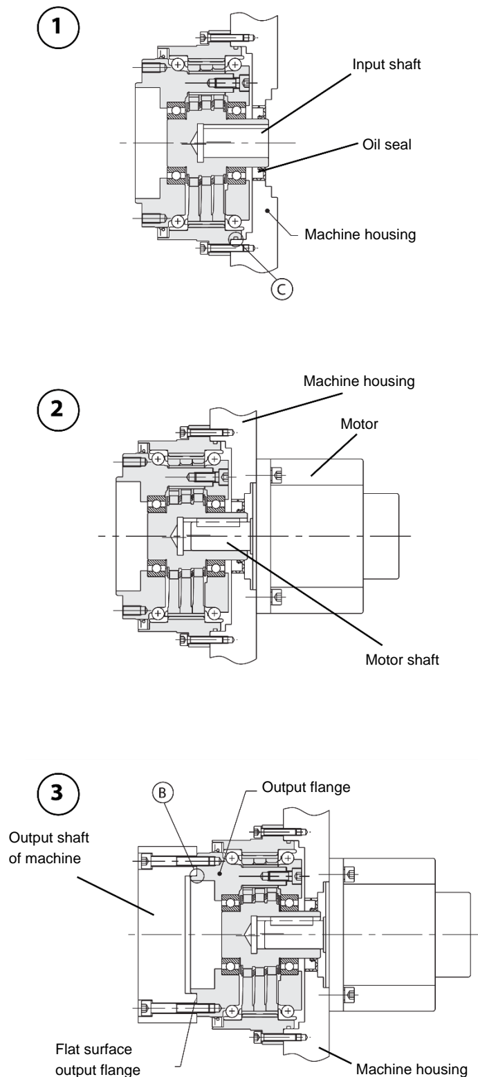
Fig. 20 F4CF-DA installation example 1
