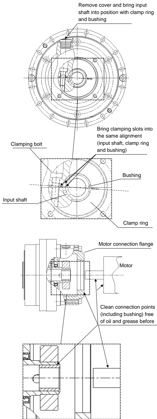
Fig. 2 Motor mounting with clamp ring
