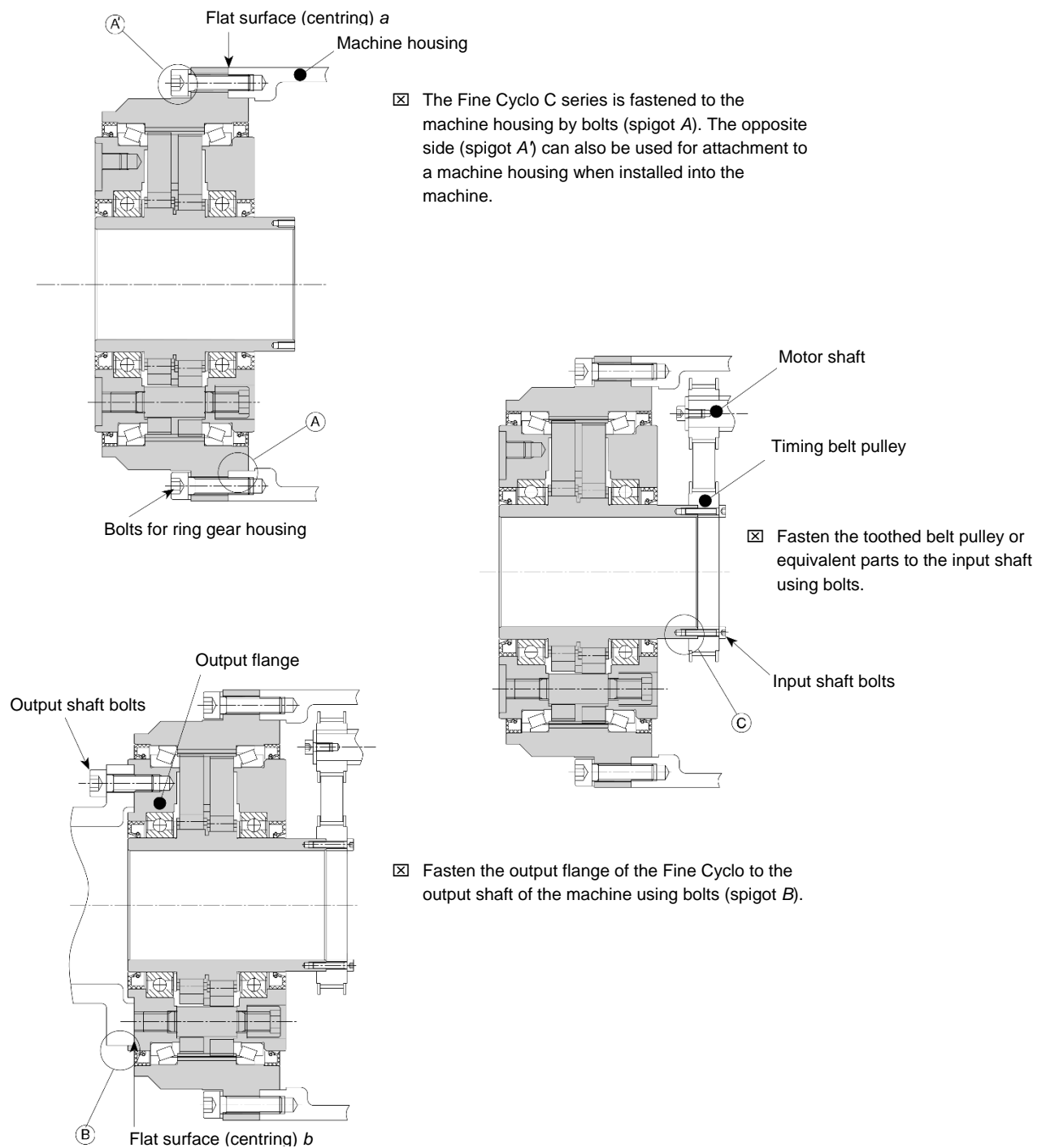
Fig. 14 F2/4(F)C-C installation example
