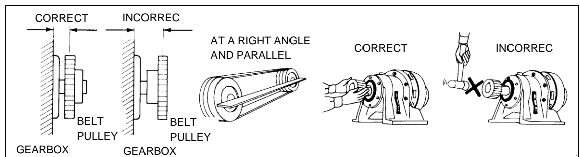
Fig. 1 Correct assembly
