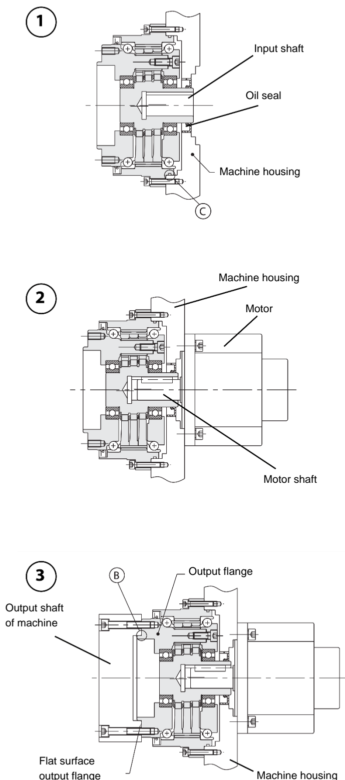
Fig. 16 Installation example 1 F4CF-D
