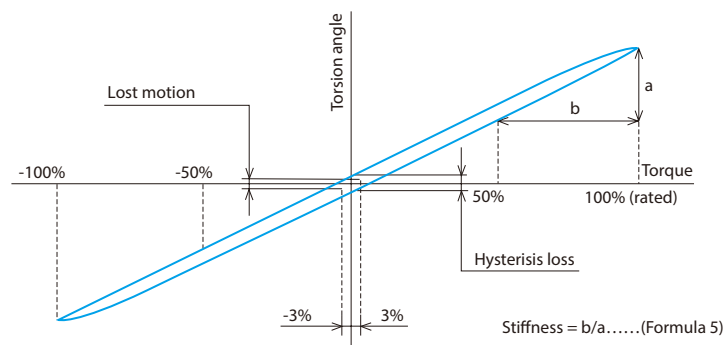
Figure 9. Hysteresis curve
