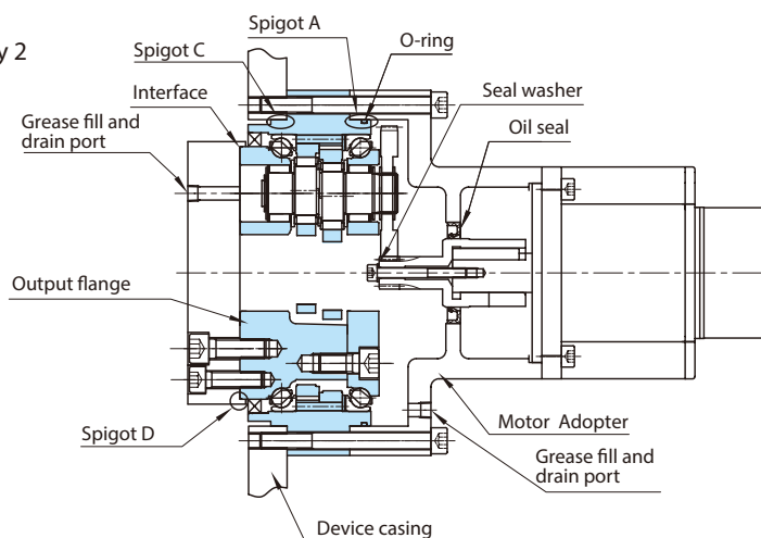
Figure 17 Assembly method
