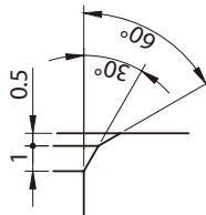
Details on Part X
